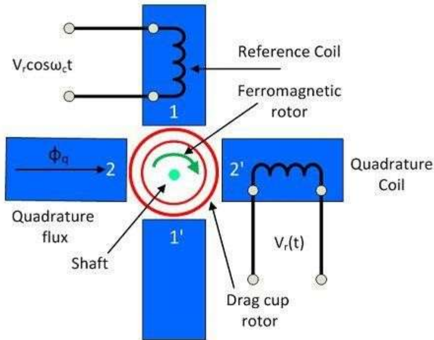
A.C Tachometer Generator
