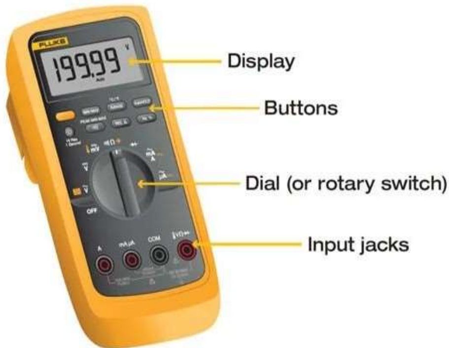
(DIGITAL MULTIMETER)
