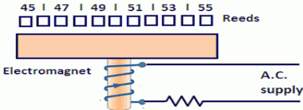
Viberating reed type frequency meter
