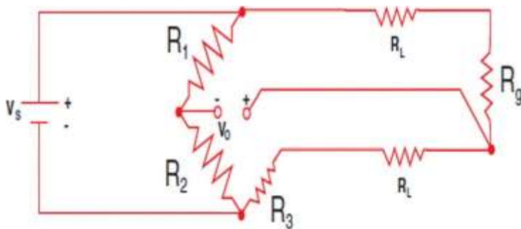
Fig.6. Circuitry view of three wires RTD Bridge
